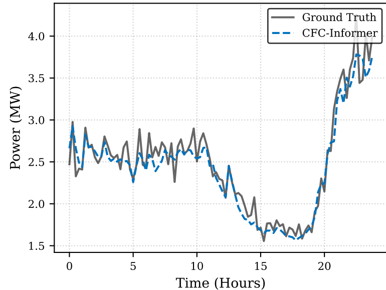
(a) Load Forecasting (MAE=0.122)
