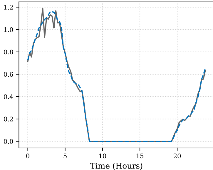
(b) PV Forecasting (MAE=0.014)
