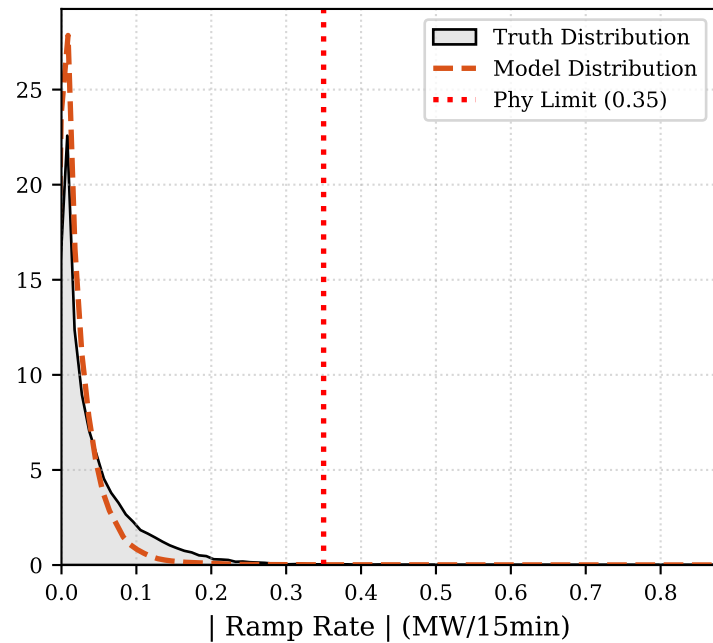
(c) Wind Dynamics Violation Rate: 0.47%
