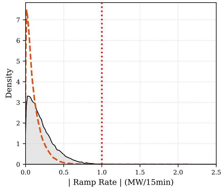
(a) Load Dynamics Violation Rate: 0.07%
