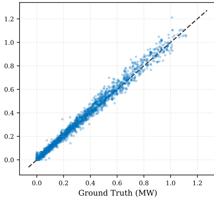
(b) PV Regression ( R^2=0.992 )
