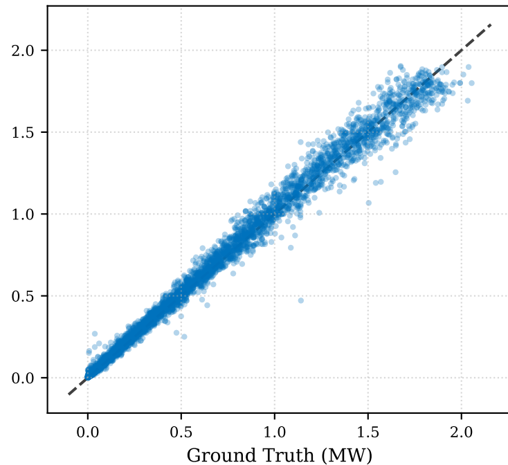
(c) Wind Regression ( R^2=0.989 )
