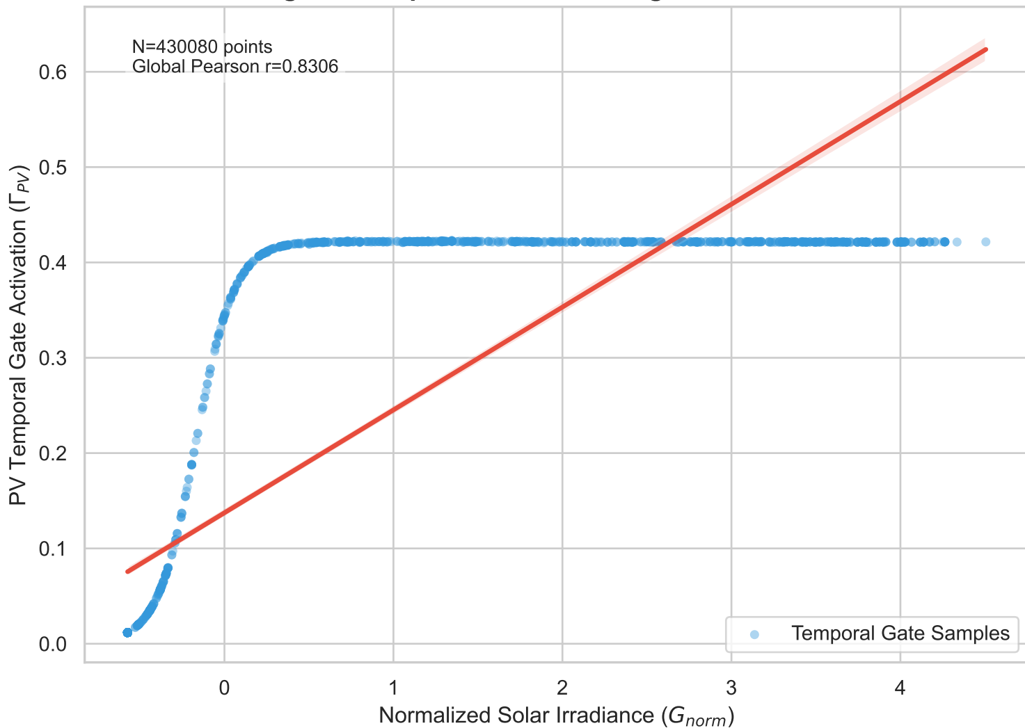
Figure 3: Supervised Causal Alignment in PGCC
