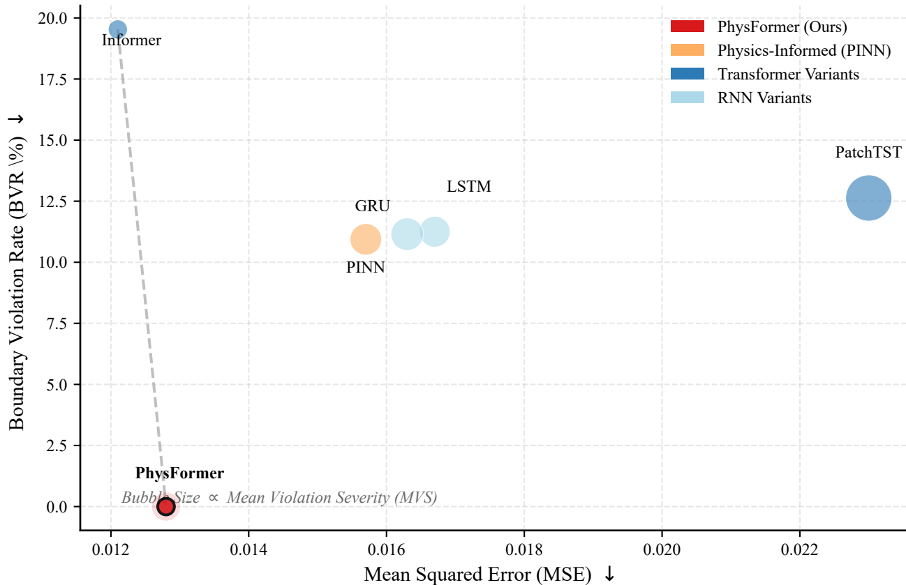
Fig. 5: Accuracy-Compliance Pareto Frontier (Bubble Size = MVS)
