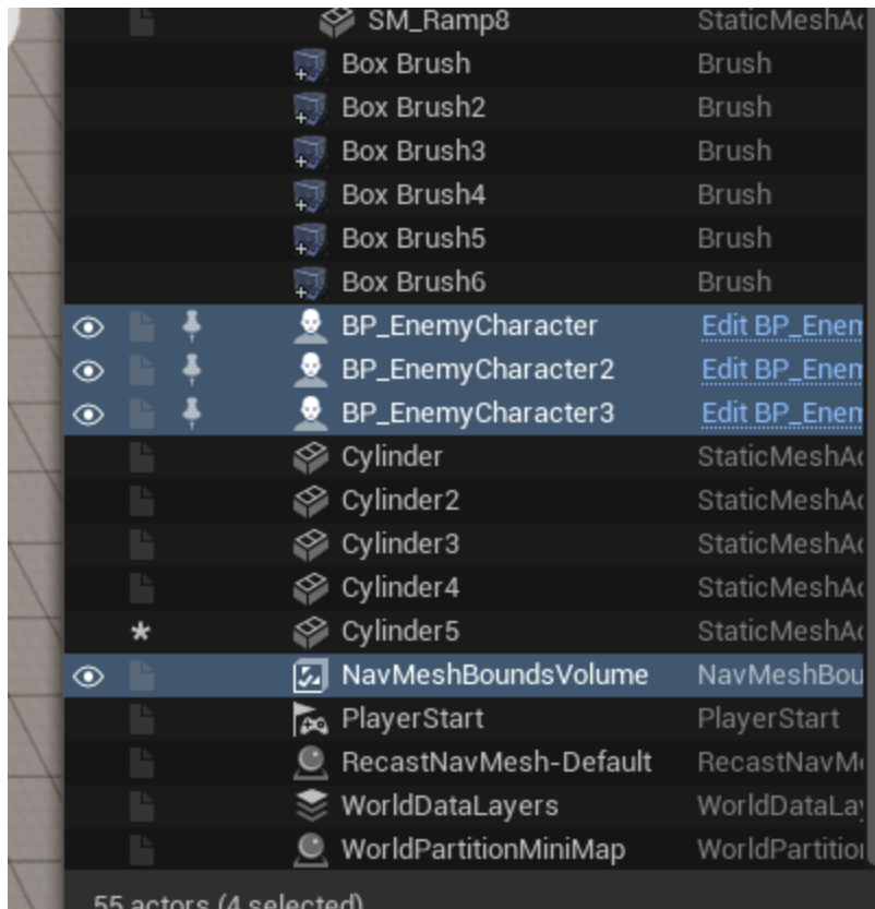
World Outliner — Showing the three BP_EnemyCharacter instances and the NavMesh Bounds Volume
