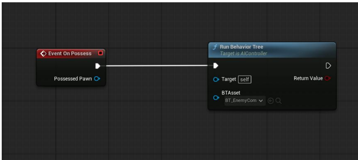
BP_EnergyAIController — OnPossess / RunBehaviorTree graph
