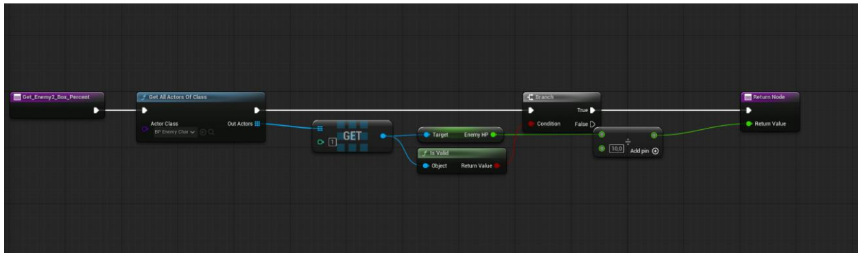
WBP_HUD — Binding function for at least one progress bar (Graph view)
