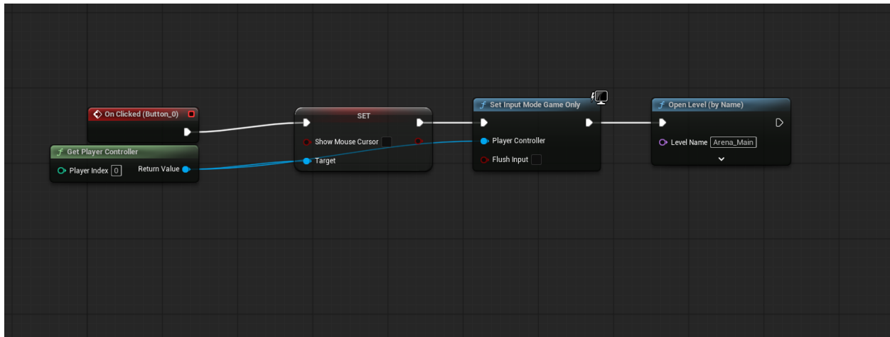
WBP_GameOver — Restart button OnClicked graph (Open Level call)
