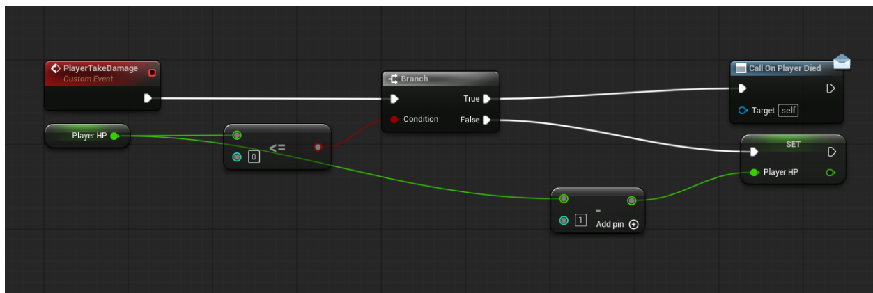
BP_ThirdPersonCharacter — TakeDamage / PlayerHP logic and death event
