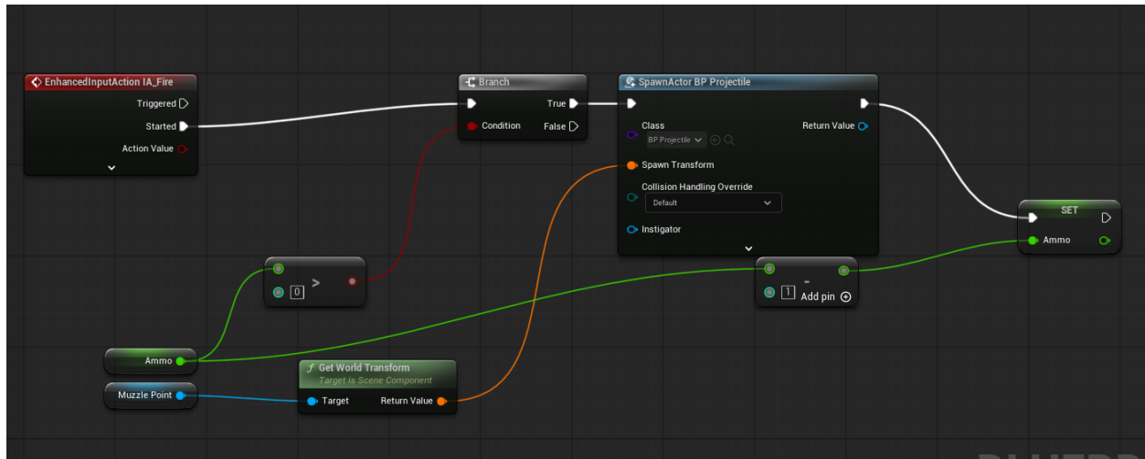
BP_ThirdPersonCharacter — Fire input event graph (ammo check → spawn projectile → decrement ammo)
