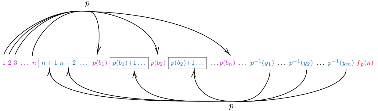
Fig. 2.3: Visualization of f_p(n)
