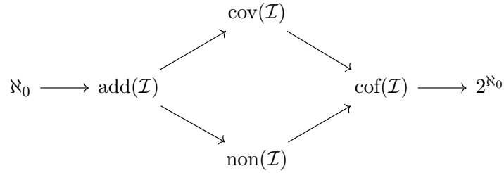
Fig. 1.2: Theorem 1.3
