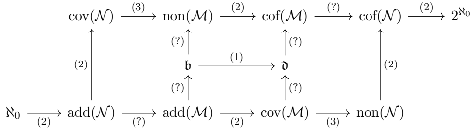
Fig. 1.1: Cichoń's Diagram (w/ clickable hyperlinks)
