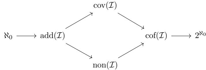
Fig. 2: Theorem 1.1
