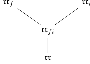
Fig. 4: Narrowed Hasse Diagram
