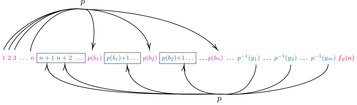
Fig. 5: Visualization of f_p(n)
