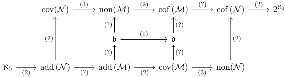
Fig. 1.1: Cichoń's Diagram (with clickable hyperlinks)
