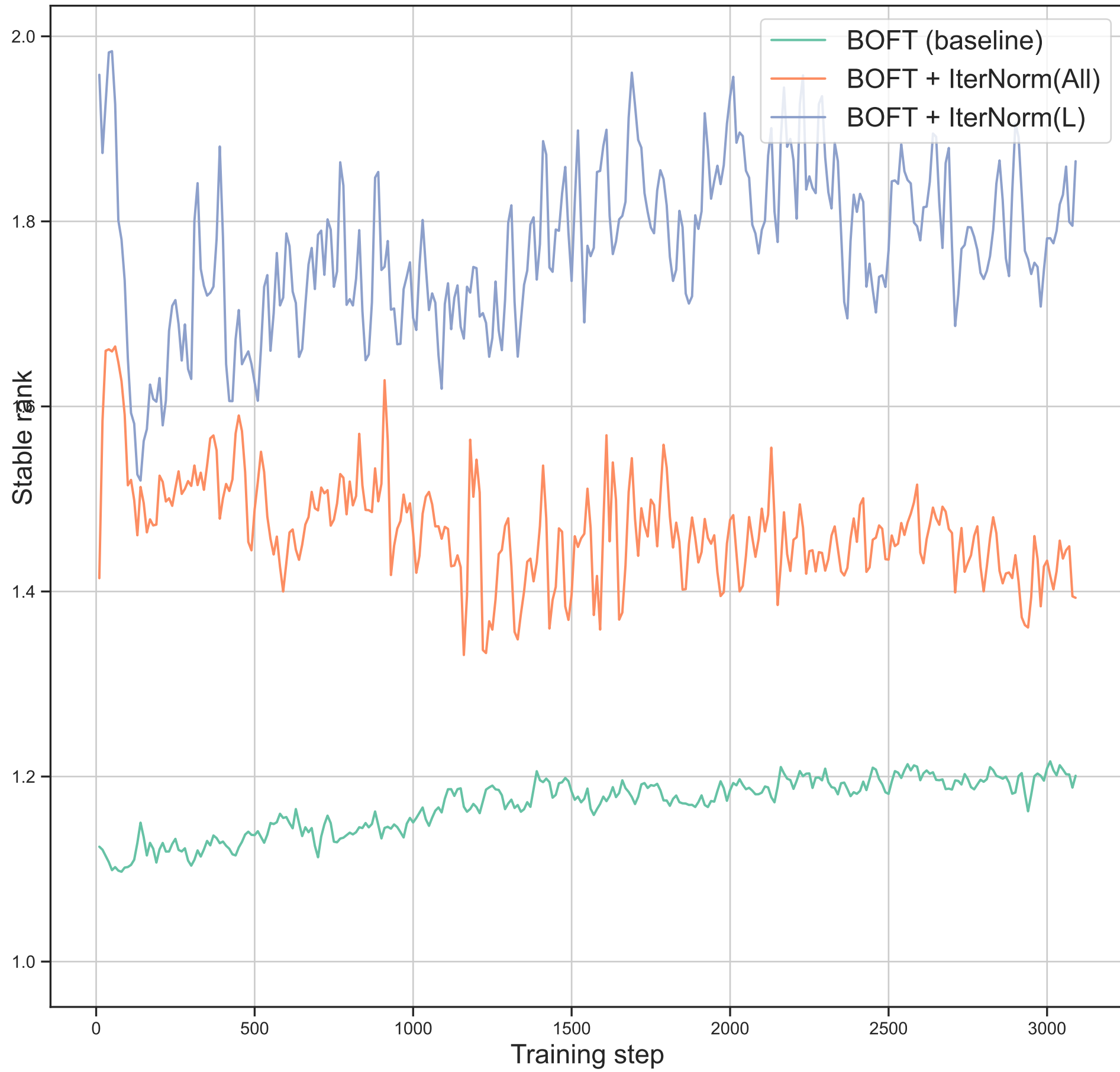
Method: BOFT
