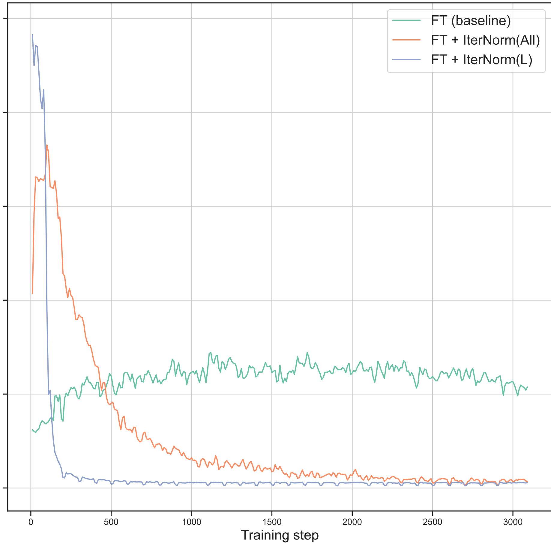
Method: FT
