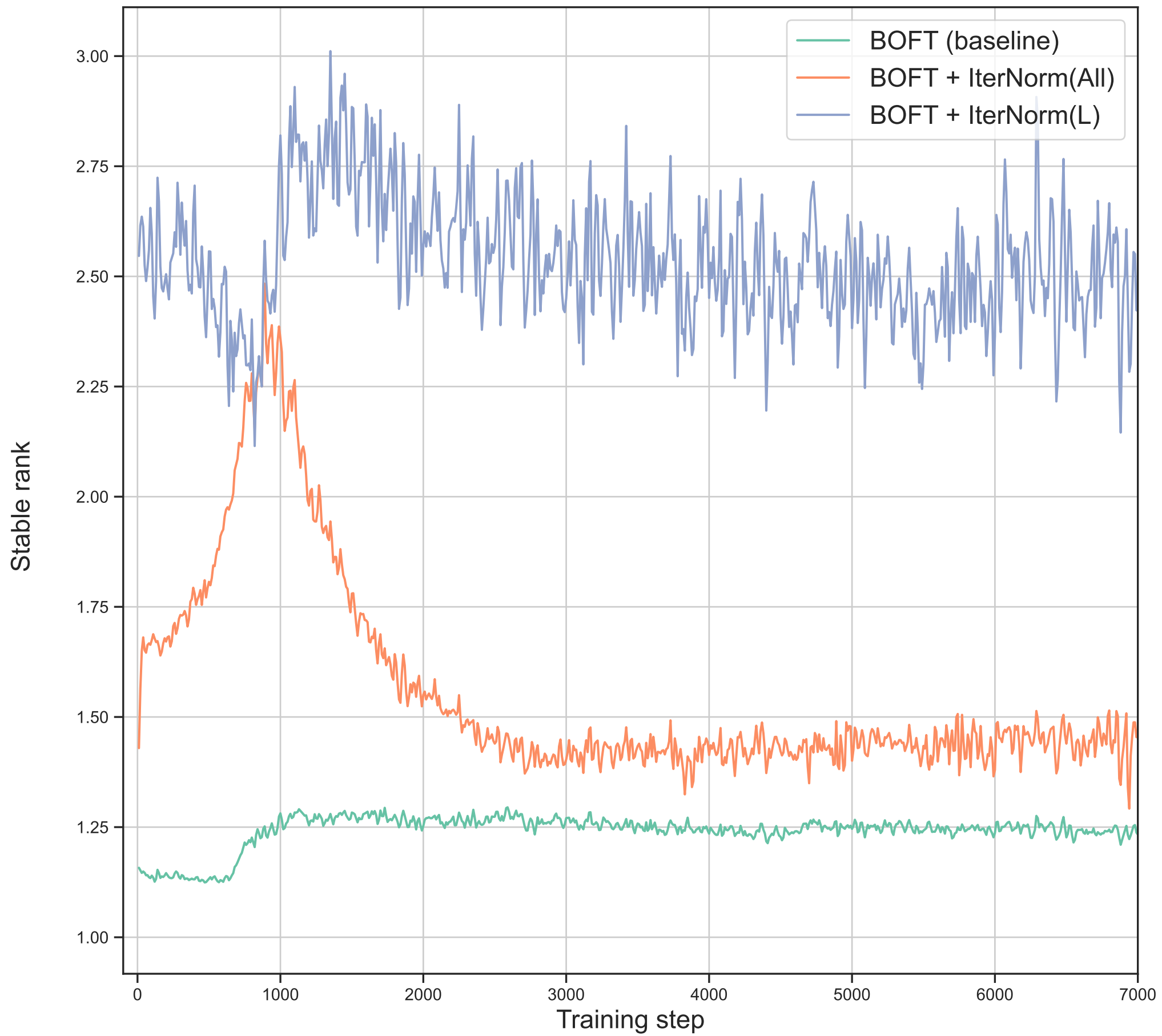
Method: BOFT
