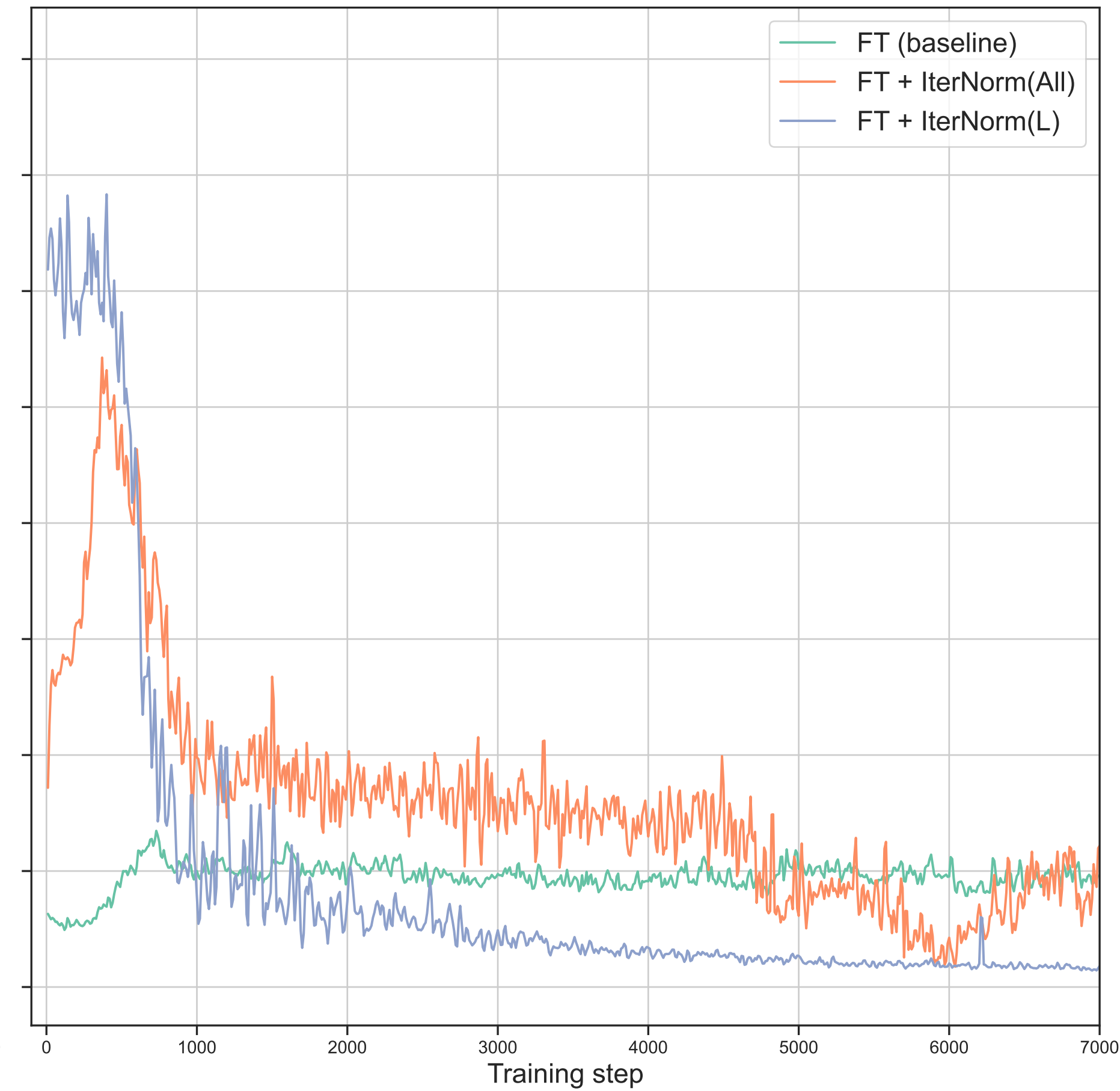
Method: FT
