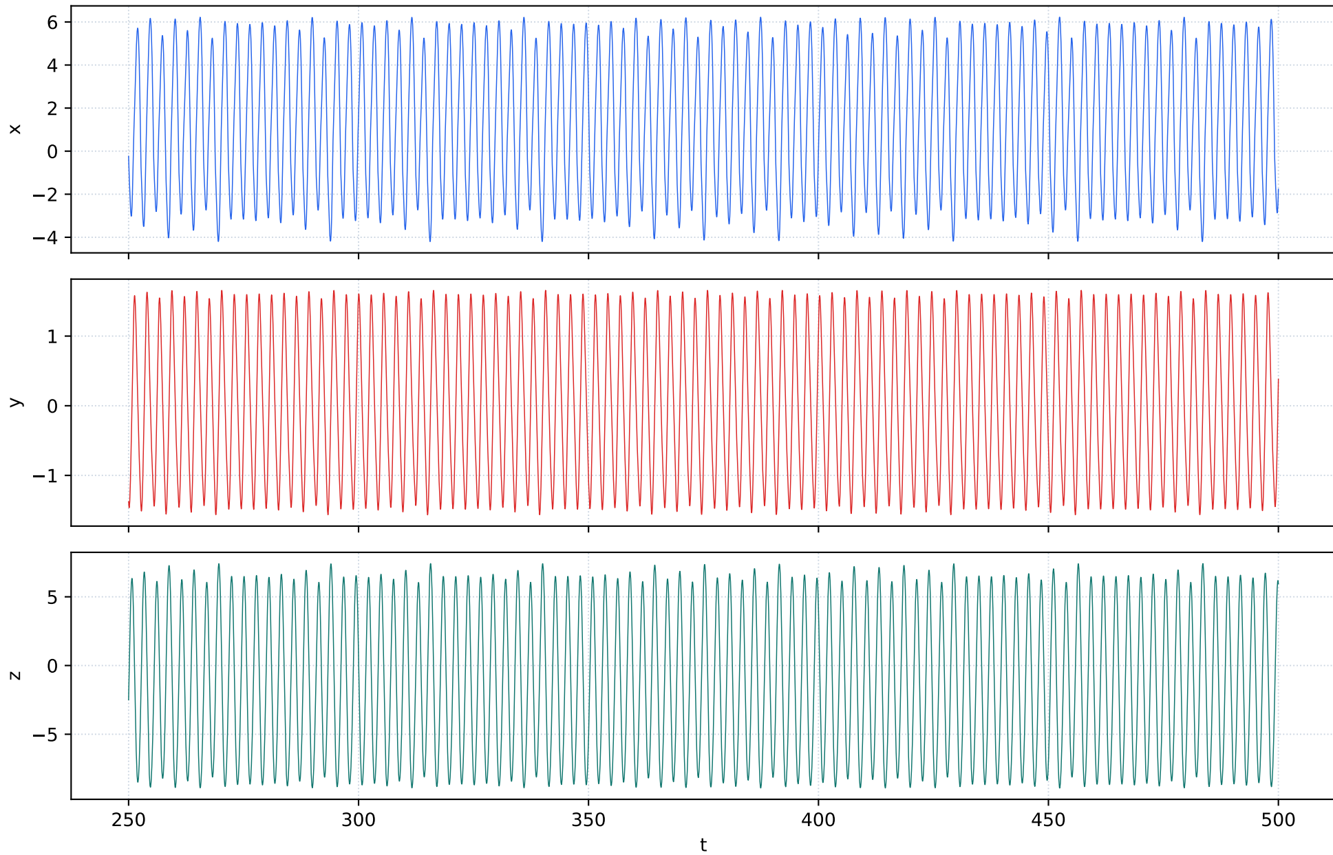
danca2017_chua_fractional_saturation_q09998 | diagnostic_X0 Danca 2017 | q=0.9998 | h=0.01 | ABM | native_full_history_abm
