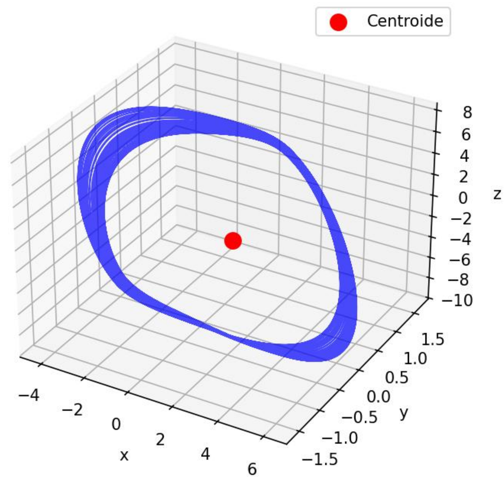
Atractor 3D Post-Transitorio
