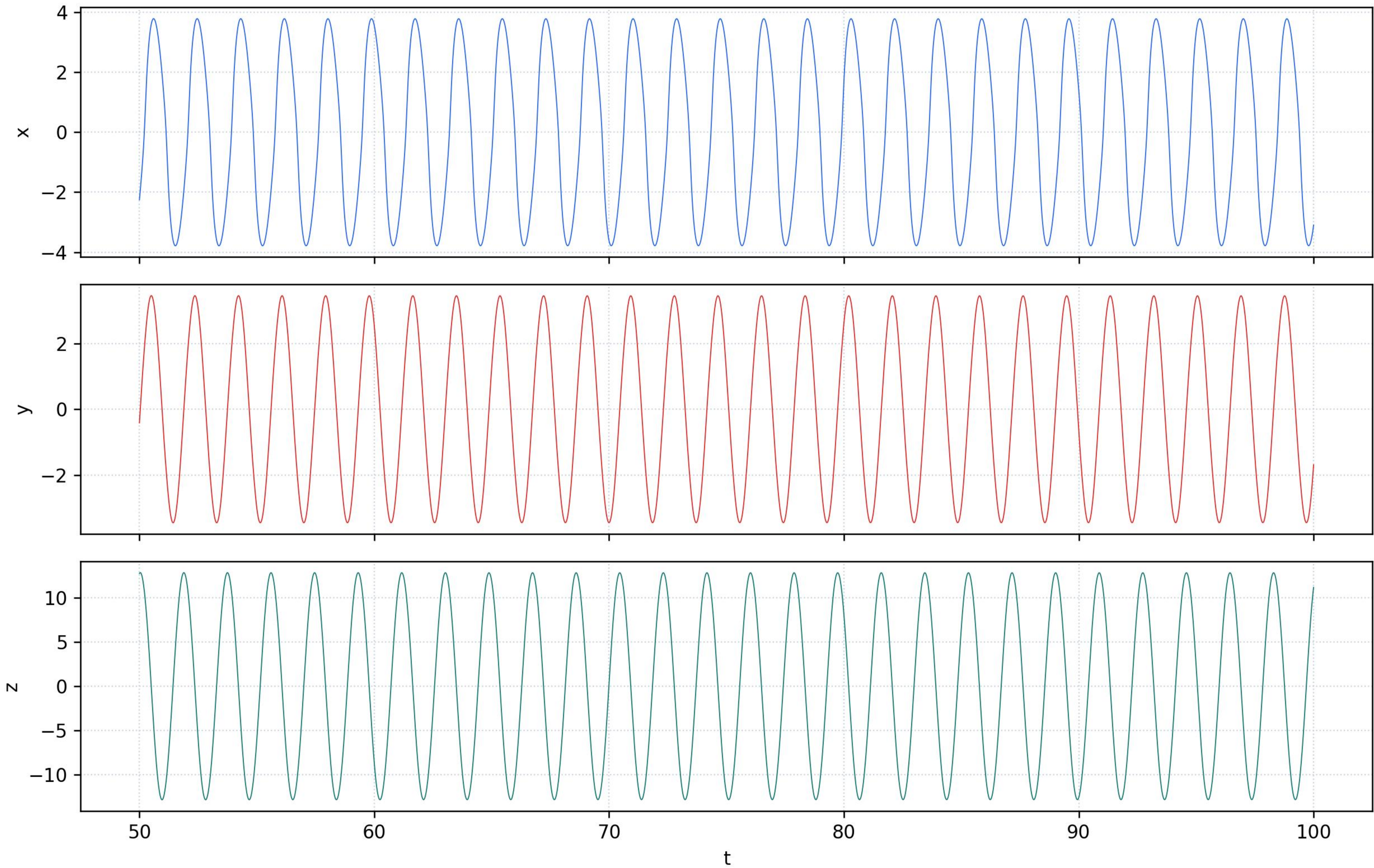
wu2023_chua_fractional_arctan_q099 | x0_minus Wu et al. 2023 | q=0.99 | h=0.01 | ADM_WU2023 | adm_local_reproduction
