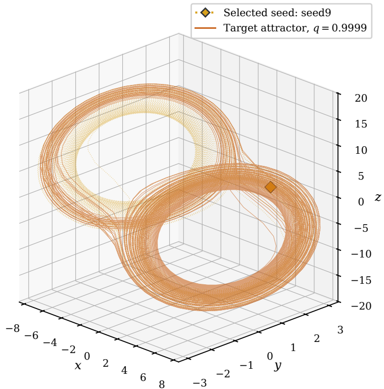
Fractional IVP from seed9
