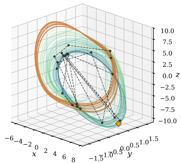
Proposed causal continuation
