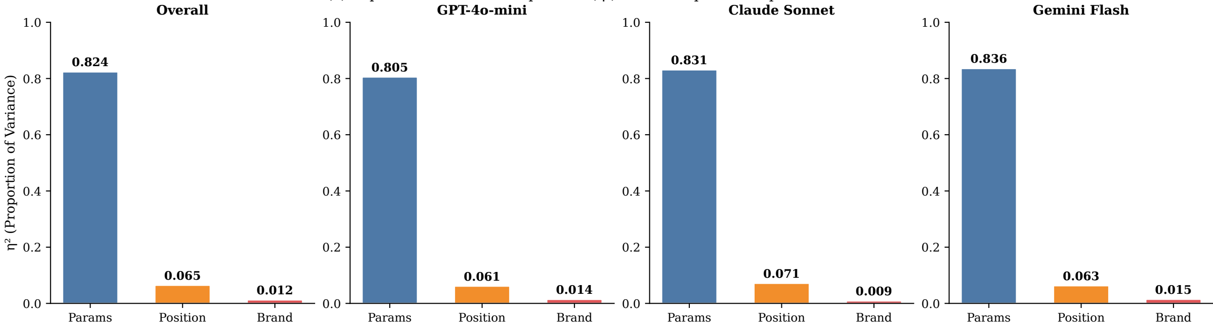
(e) Exp 1d: Variance Decomposition ( \eta^2 ) — rank \sim params + position + brand
