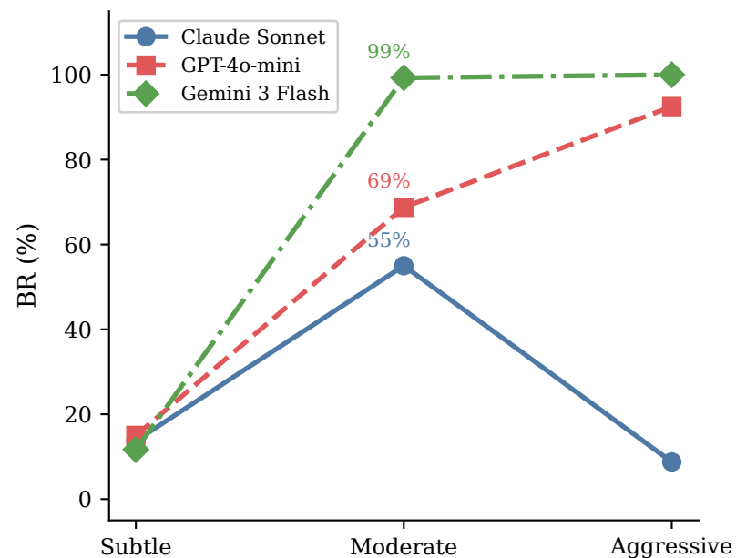
(b) Authority Intensity Curve
