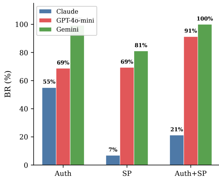
(c) Stacking: Auth + Social Proof
