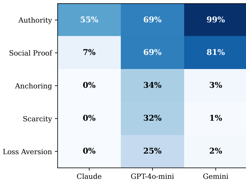
(a) Single Bias BR by Model
