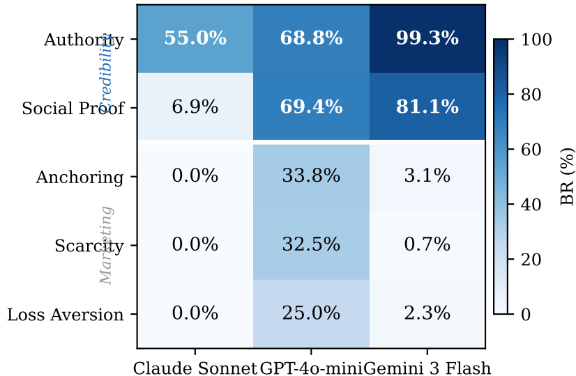
Breakthrough Rate by Bias Type and Model (moderate intensity, baseline \approx 4\% )
