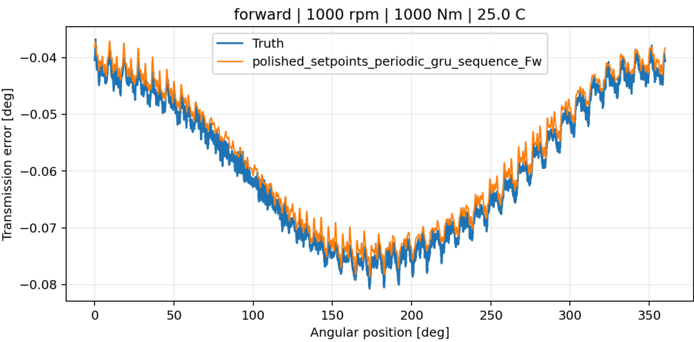
polished_setpoints_periodic_gru_sequence_Fw measured-versus-predicted TE curve
