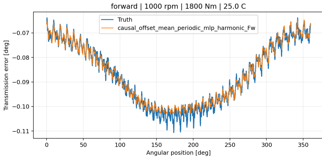
causal_offset_mean_periodic_mlp_harmonic_Fw measured-versus-predicted TE curve
