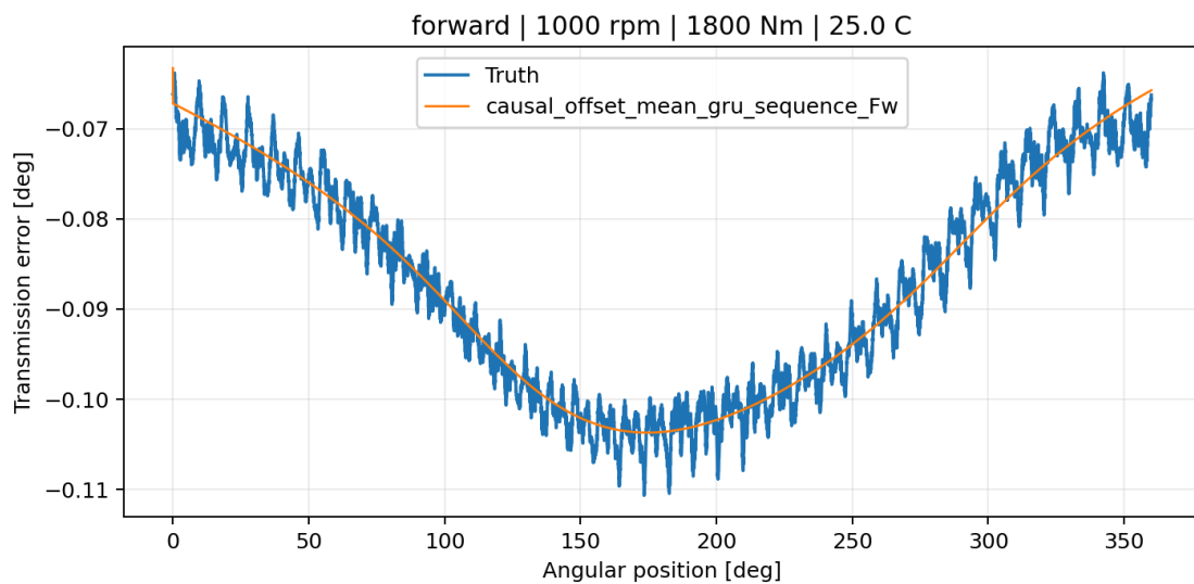
causal_offset_mean_gru_sequence_Fw measured-versus-predicted TE curve
