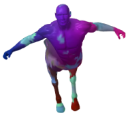
SinkHorn
