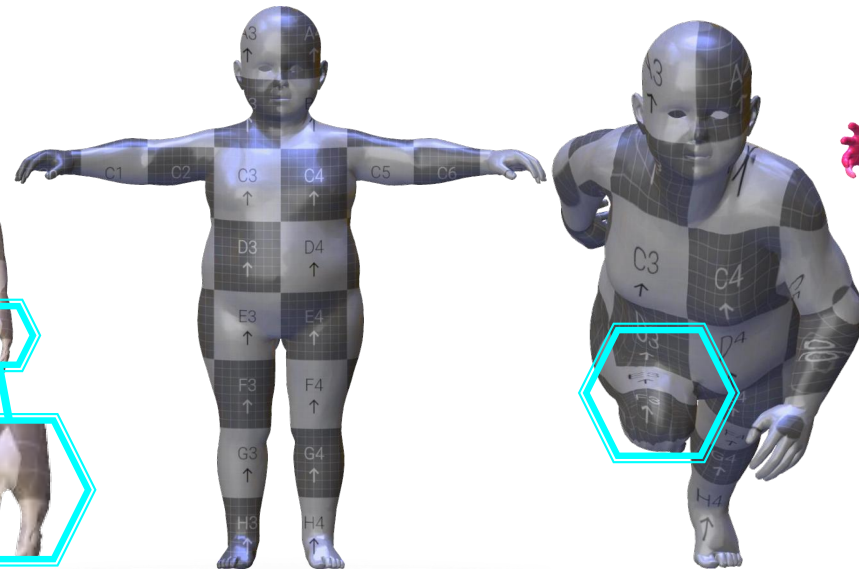
Topological Noise
