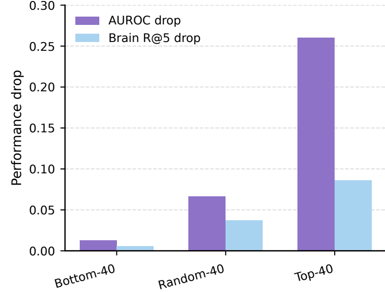
Deletion validates gate importance
