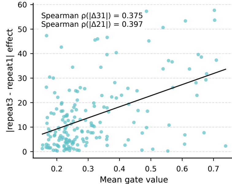
Gates track repetition effects
