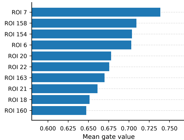
Top gated ROIs
