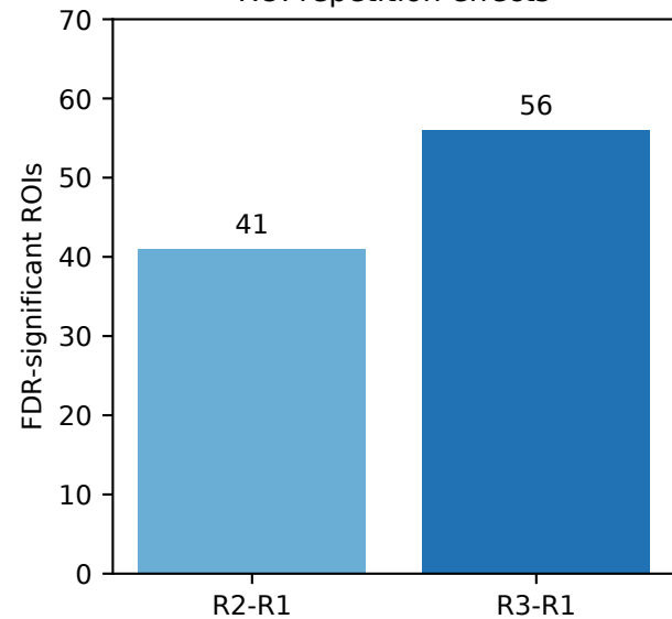
ROI repetition effects
