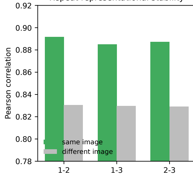
Repeat representational stability
