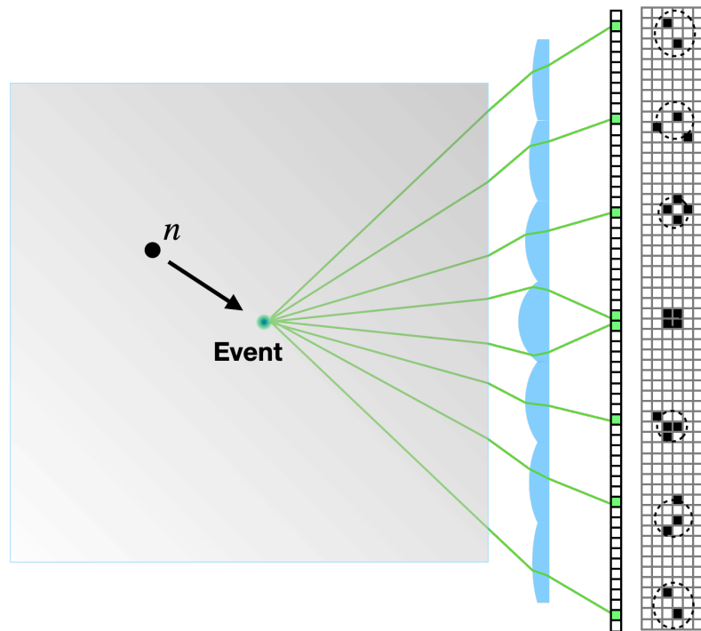
(a) Scintillator Measurement
