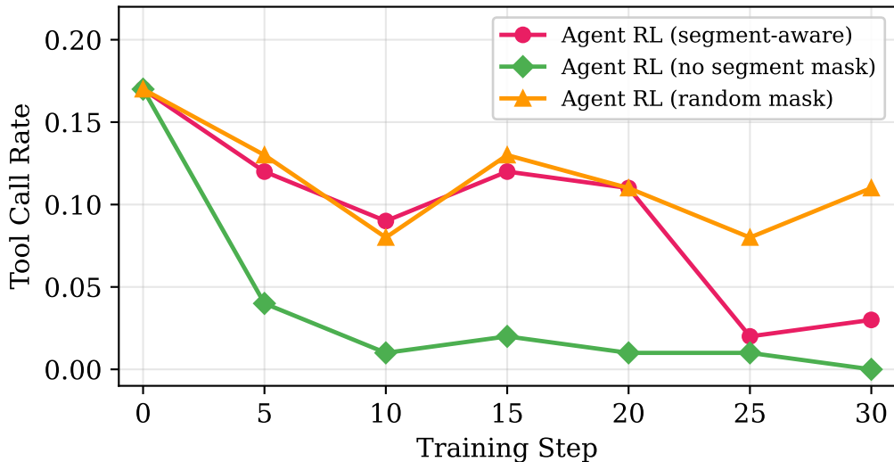
(b) Tool Call Rate over Training Steps
