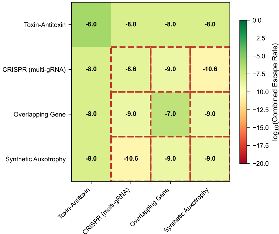
Pairwise Combination Escape Rates ( \rho = 0.01 )
