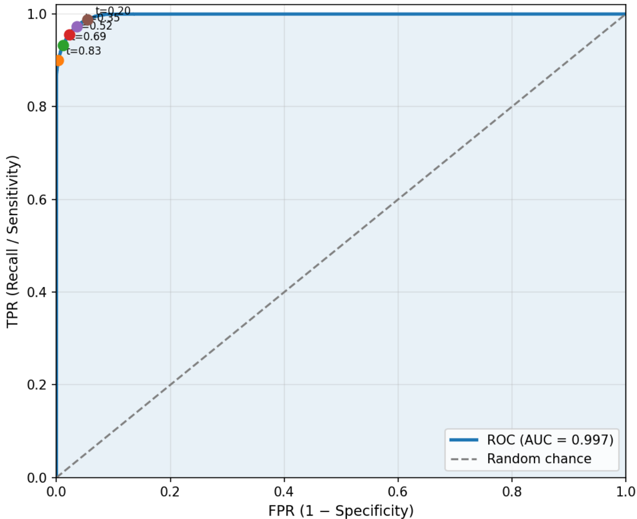
ROC Curve — Medical Insurance Classifier
