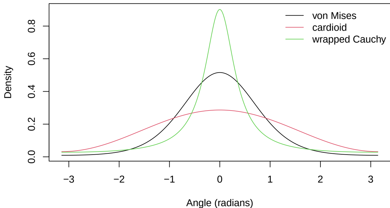
Figure 1: Three circular density families with mean direction zero.
