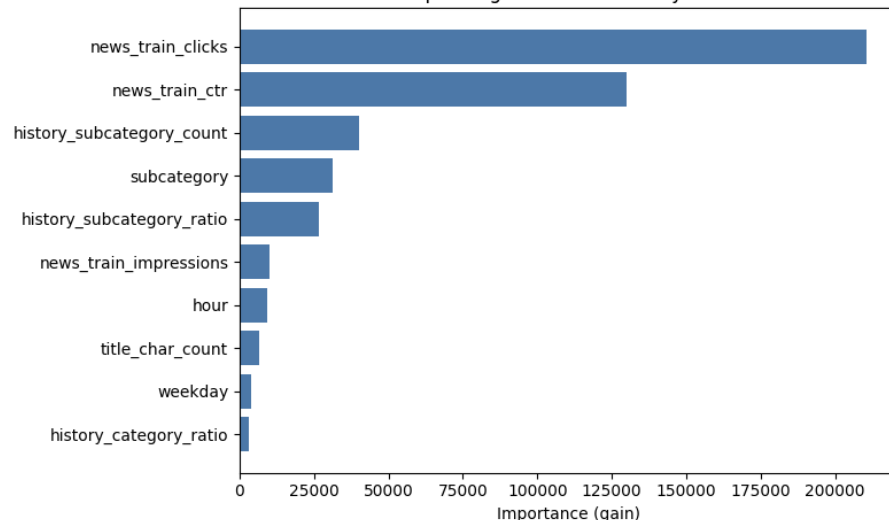
Top 10 LightGBM Features by Gain
