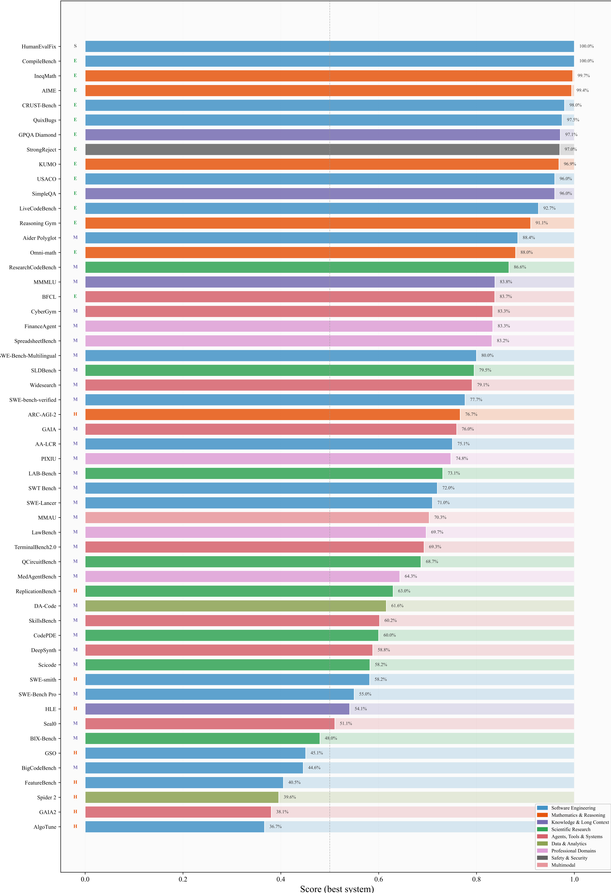
Benchmark Headroom (ranked by best score) Difficulty tier: F=Frontier (<5%), H=Hard (5-30%), M=Medium (30-70%), E=Easy (70-95%), S=Saturated (>95%)
