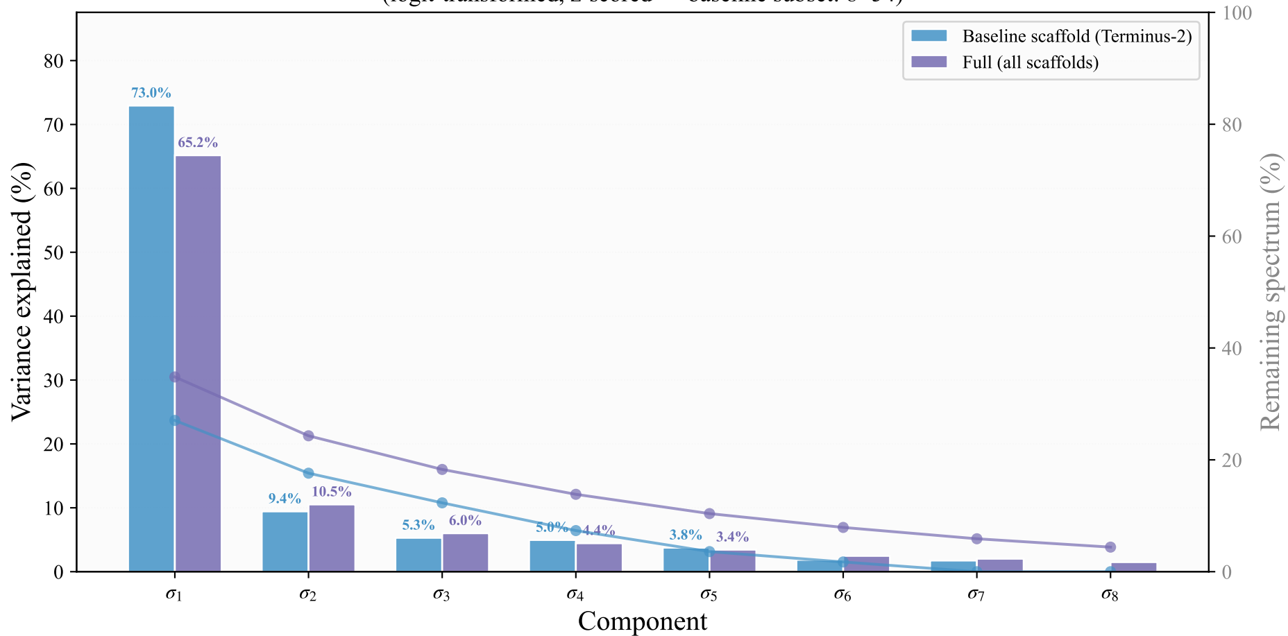
Singular value spectrum of the 16×54 benchmark matrix (logit-transformed, z-scored — baseline subset: 8×54)
