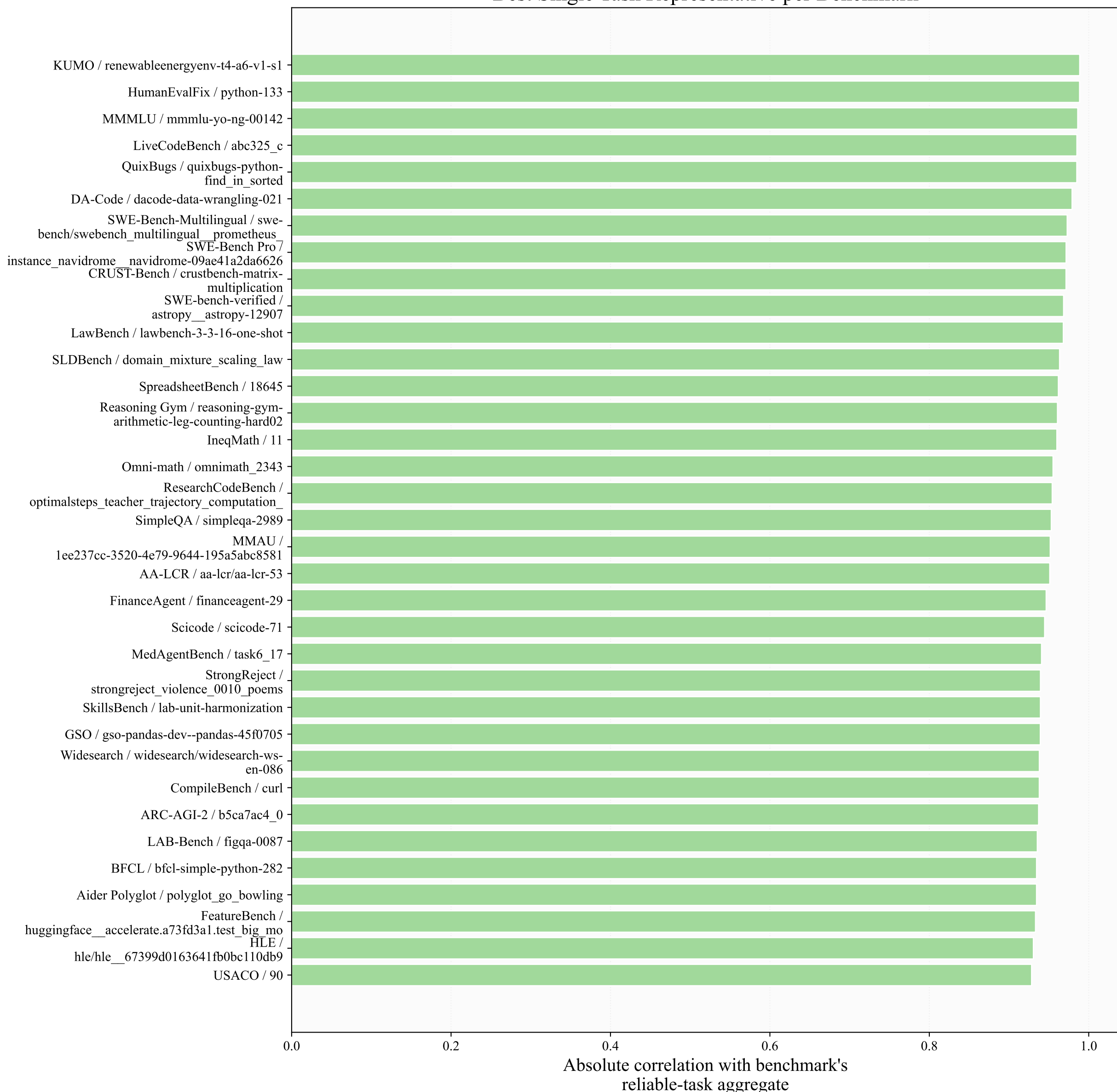
Best Single Task Representative per Benchmark
