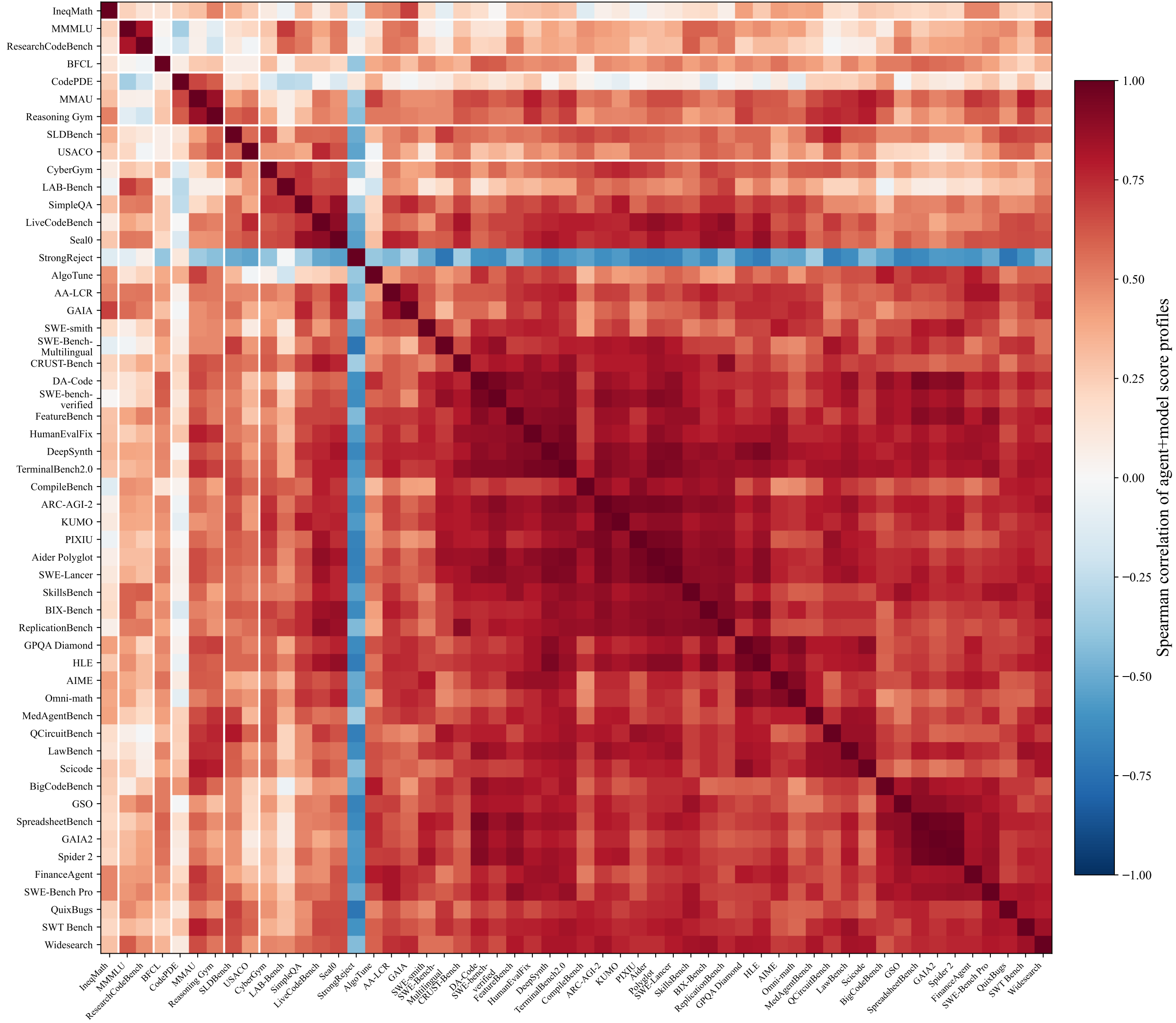
Clustered Benchmark Similarity
