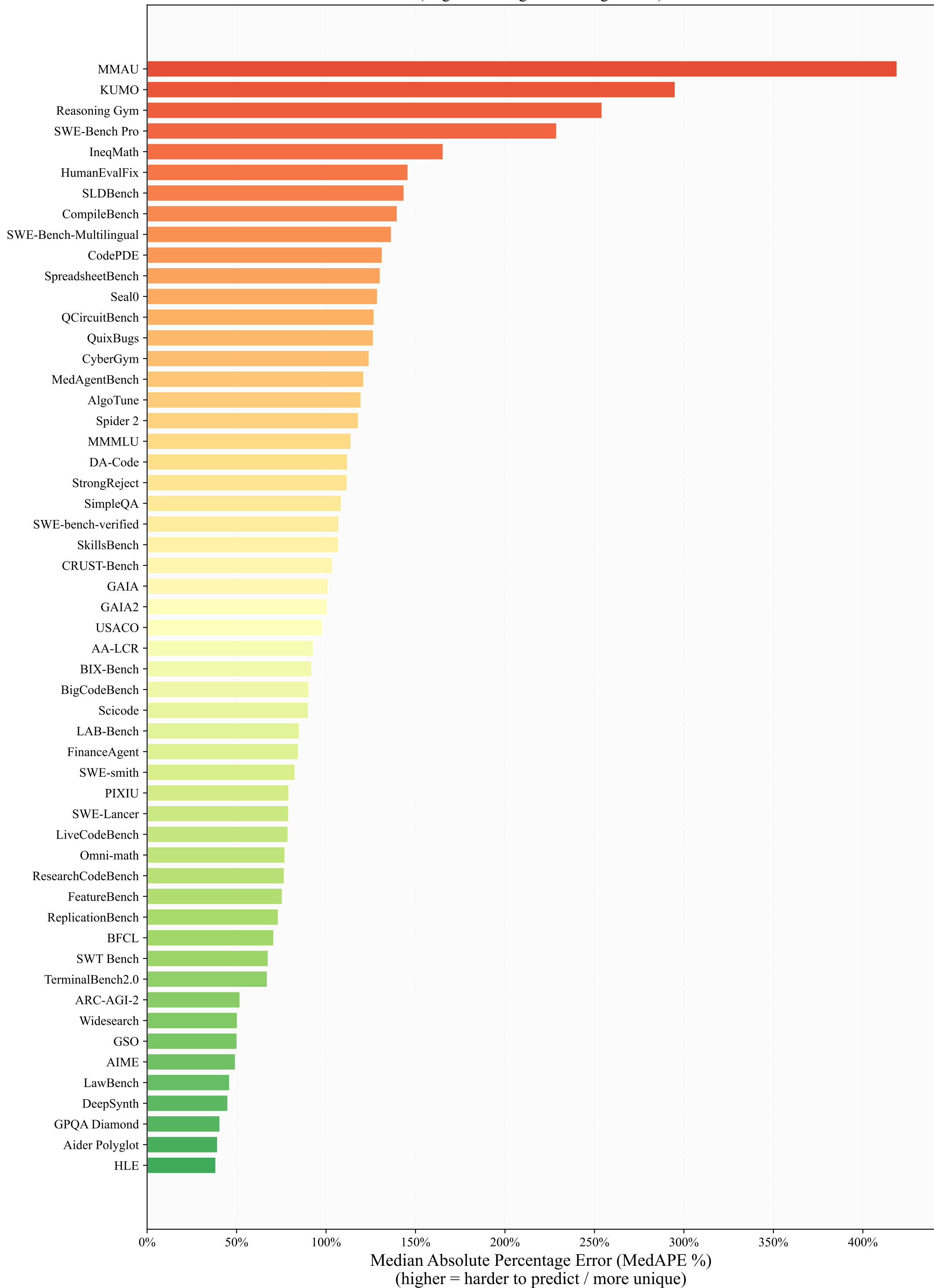
BenchPress Predictability: Per-Benchmark Holdout Error (LogitBenchReg + SVD-Logit blend)
