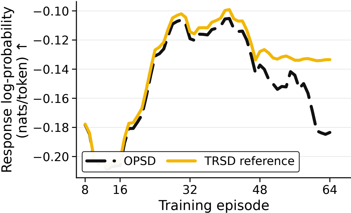
(a) TRSD reference likelihood
