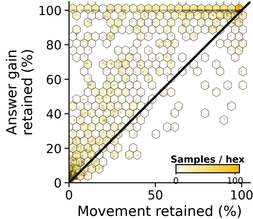
(b) Useful correction is local
