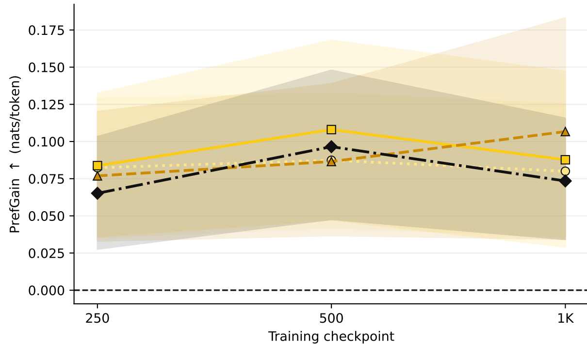
Human-preference gain
