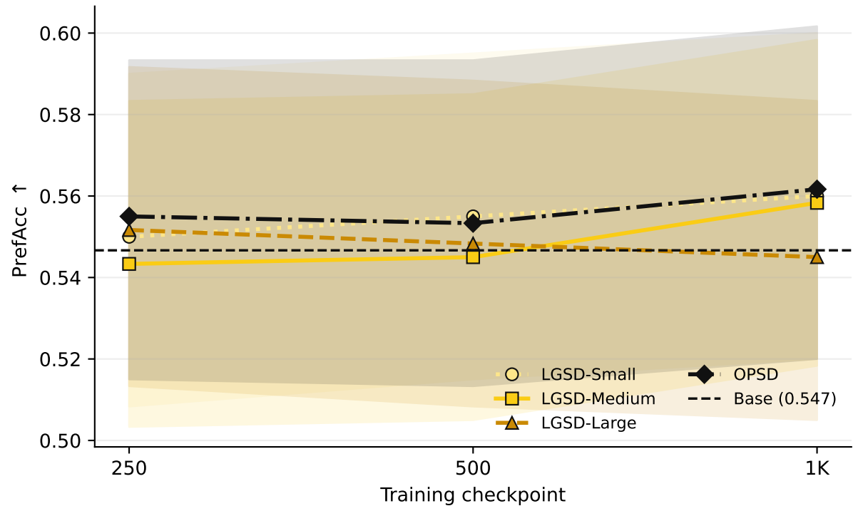
Human-preference accuracy
