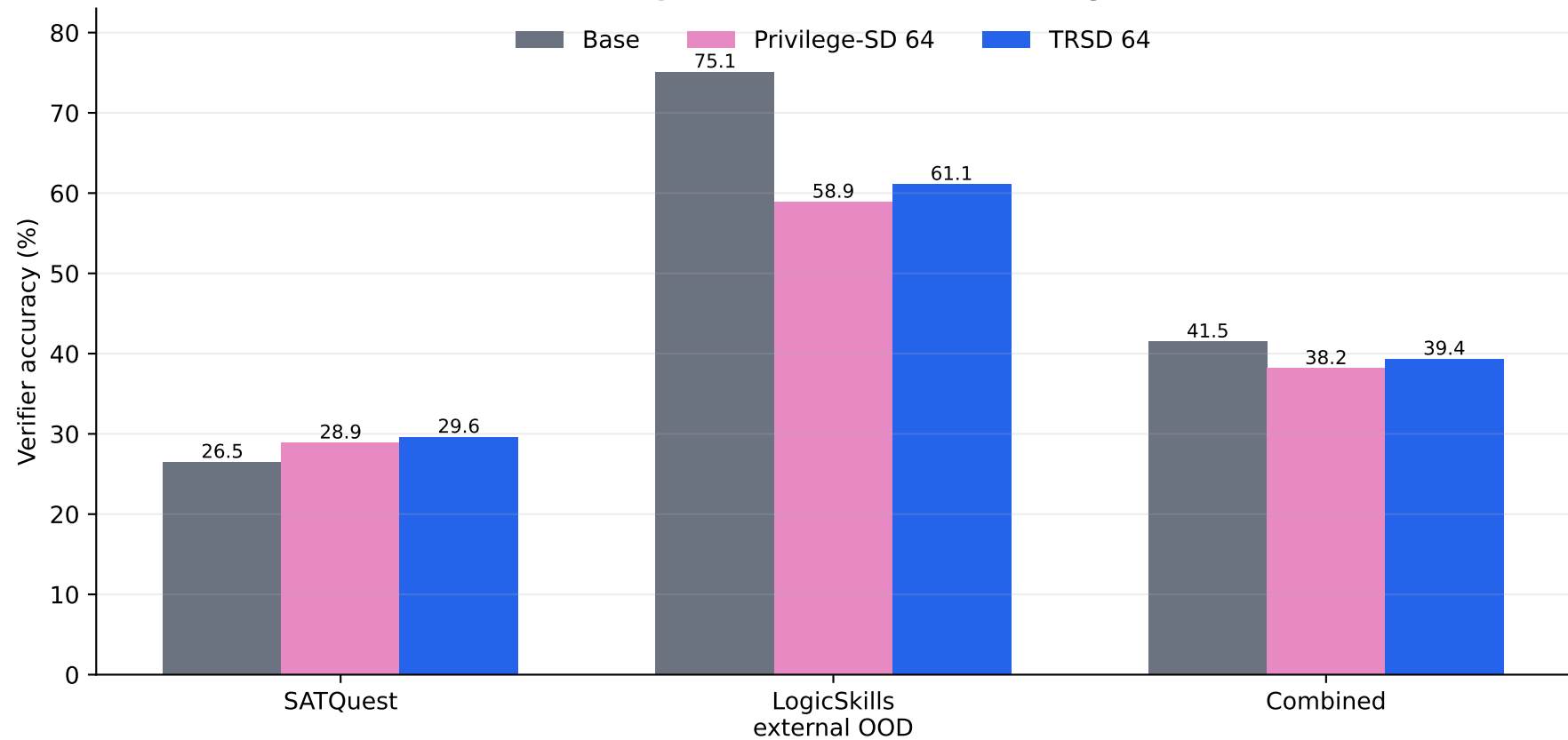
Qwen3-8B: task acquisition versus external logical retention
