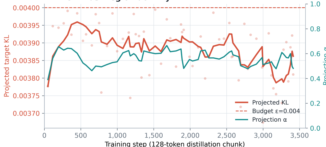
F TRSD trust-region activity
