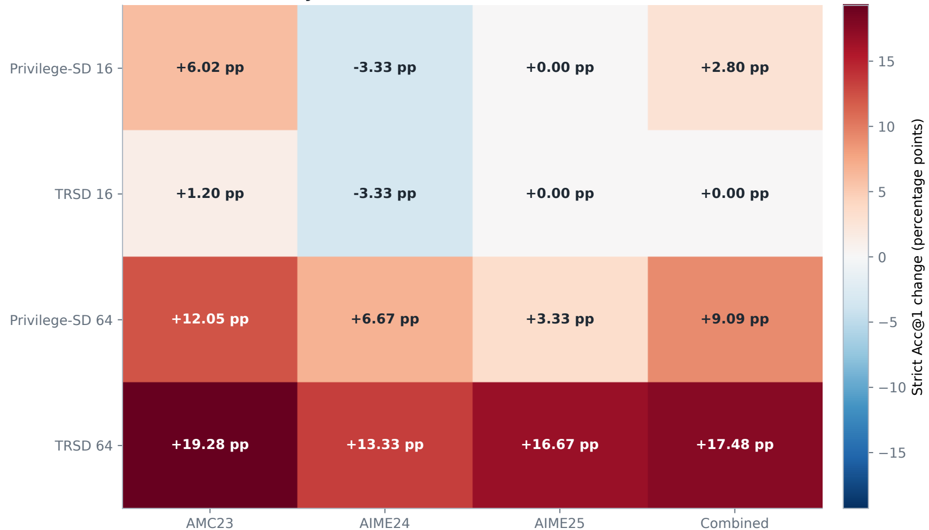
Qwen3-8B · Accuracy movement relative to Base
