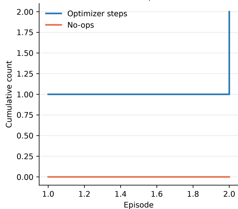
Executed updates
