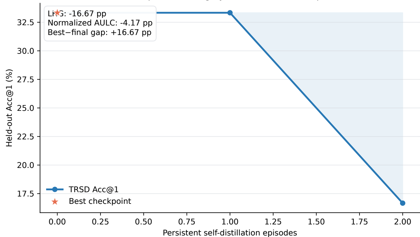
Checkpoint learning dynamics (short TRSD pilot)
