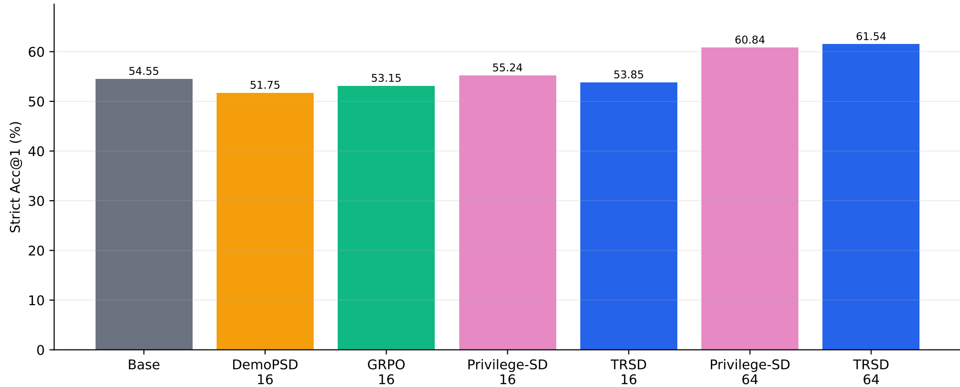
Qwen3-8B: matched DeepMath training and matched evaluation
