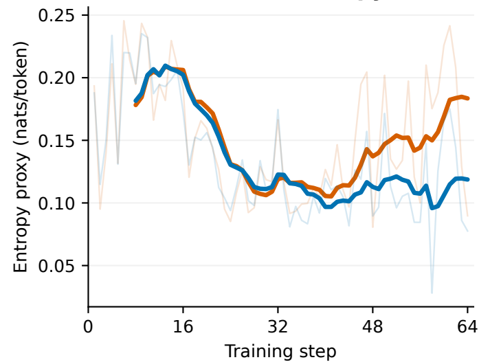
(a) Math: entropy
