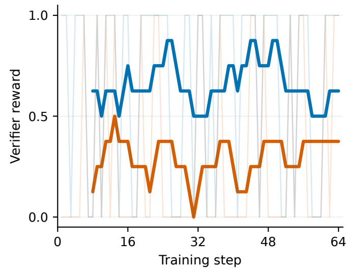
(c) Math: reward
