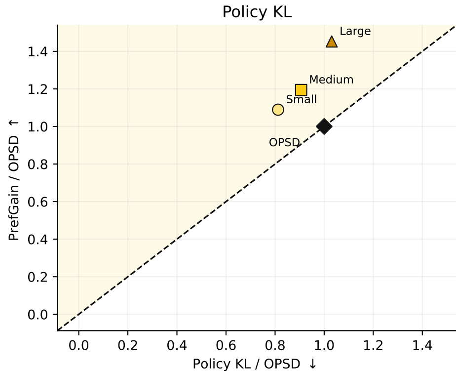
Final-checkpoint utility retained versus movement retained
