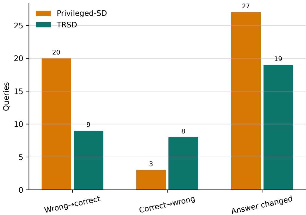
Paired behavioral transitions vs Base
