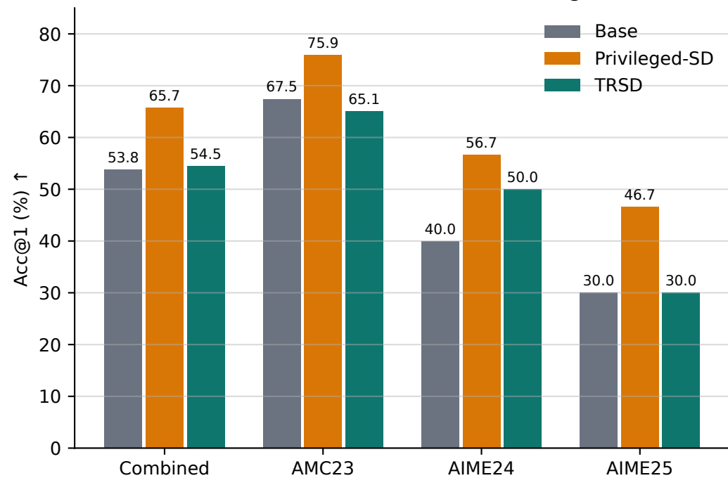
Held-out mathematical reasoning
