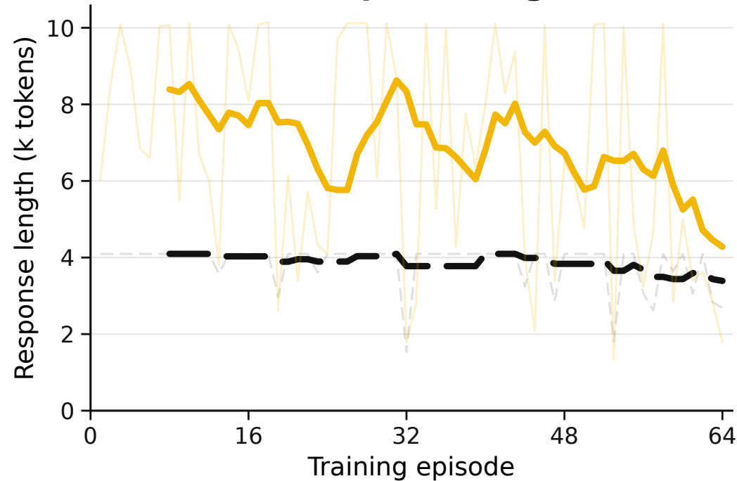
(b) Response length
