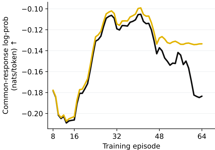
TRSD on Qwen3-8B
