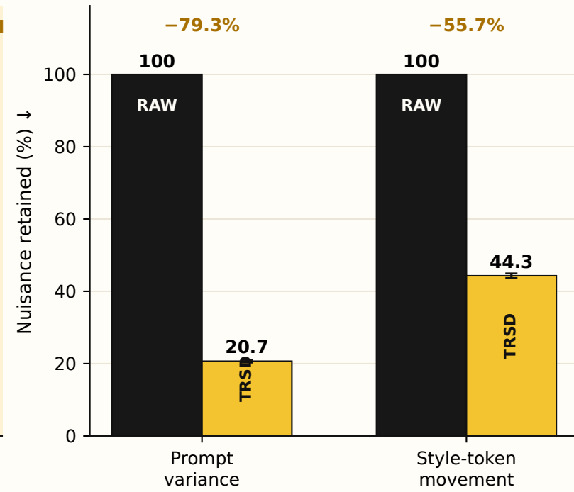
B Projection filters wrapper nuisance
