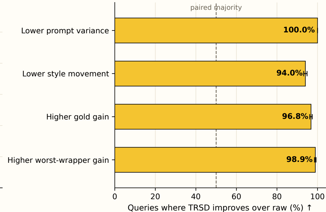
C Improvement is population-wide
