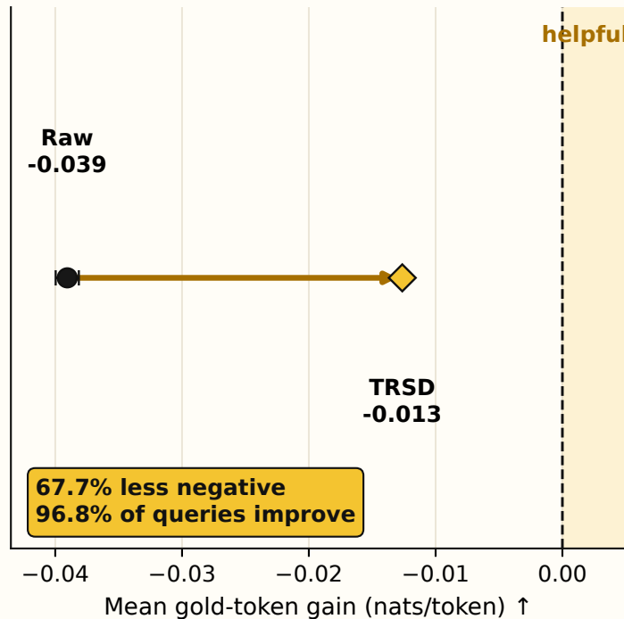
A Raw privilege is often harmful
