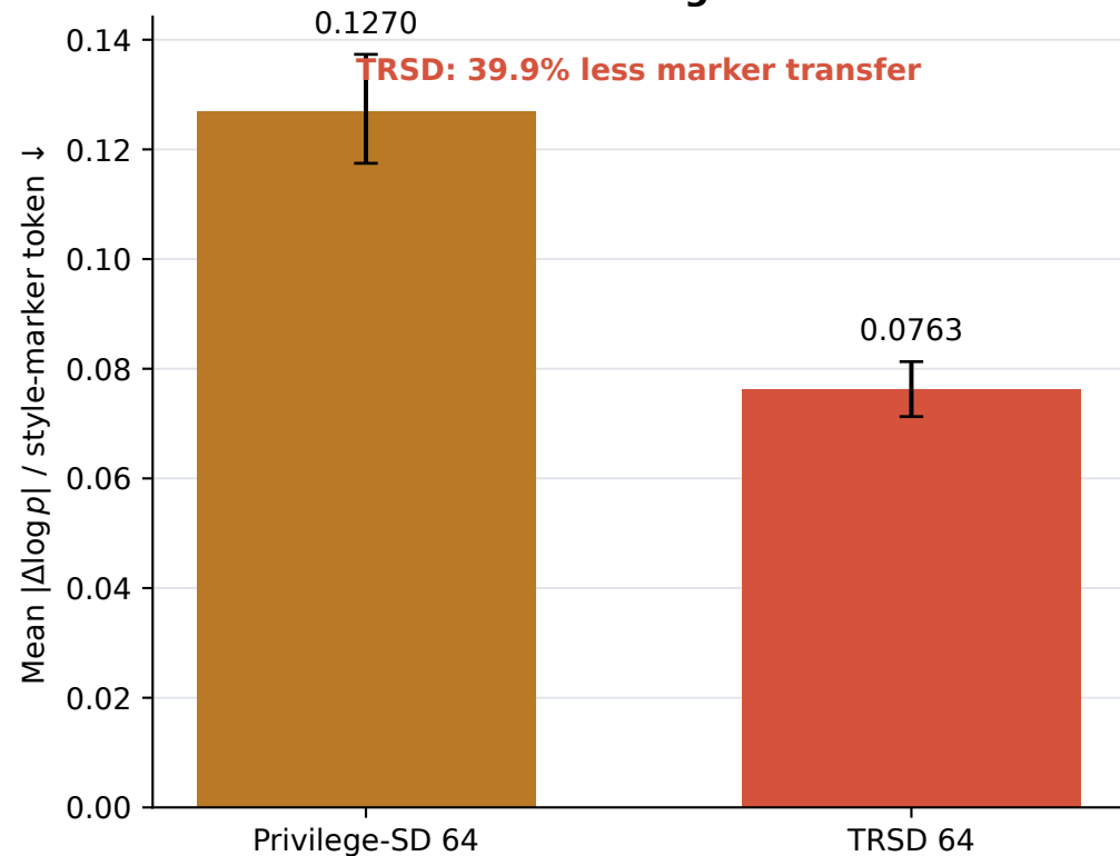
A Lexicon-conditioned diagnostic
