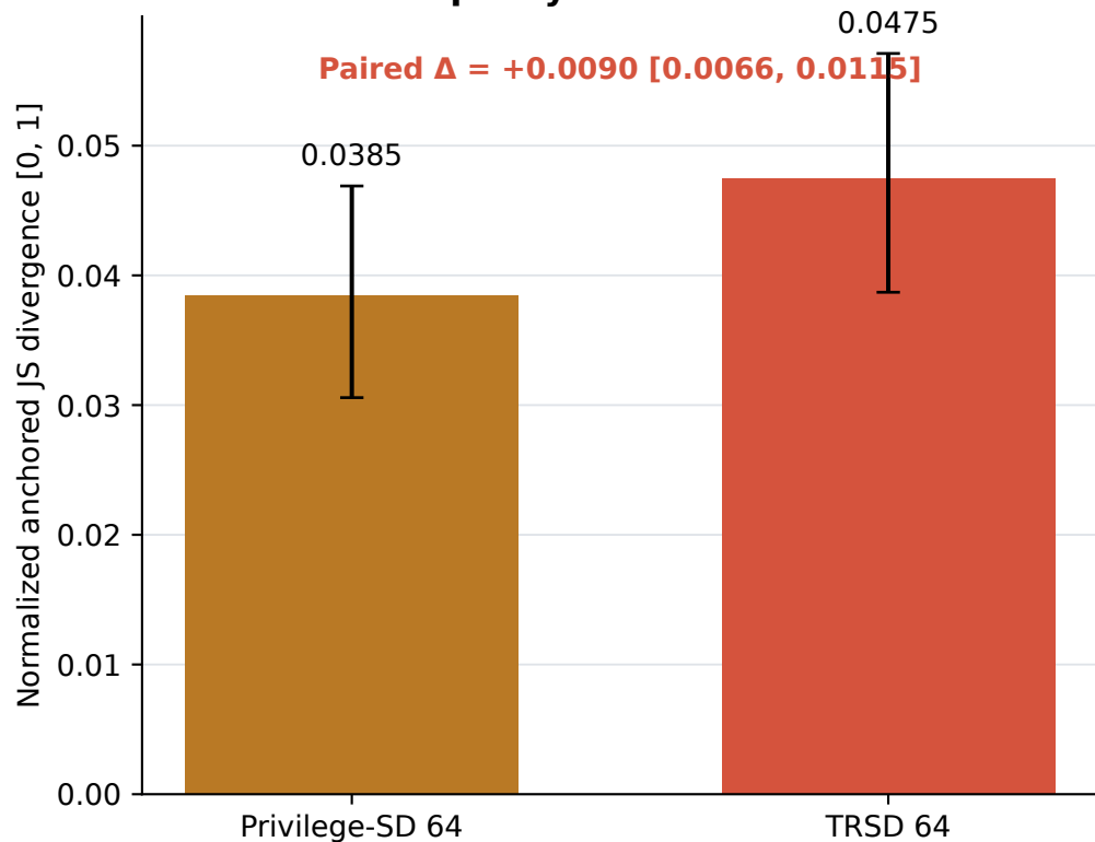
B Lexicon-free policy drift
